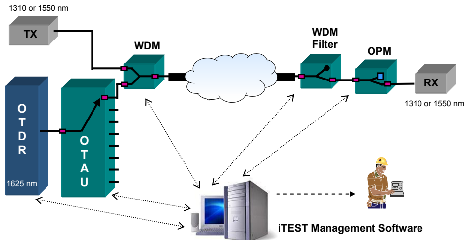
Figure 5 – iTEST Active RFTS System
