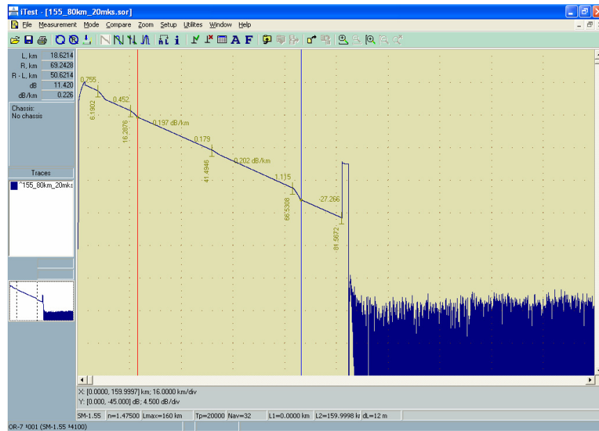
Figure 4 – OTDR Trace
